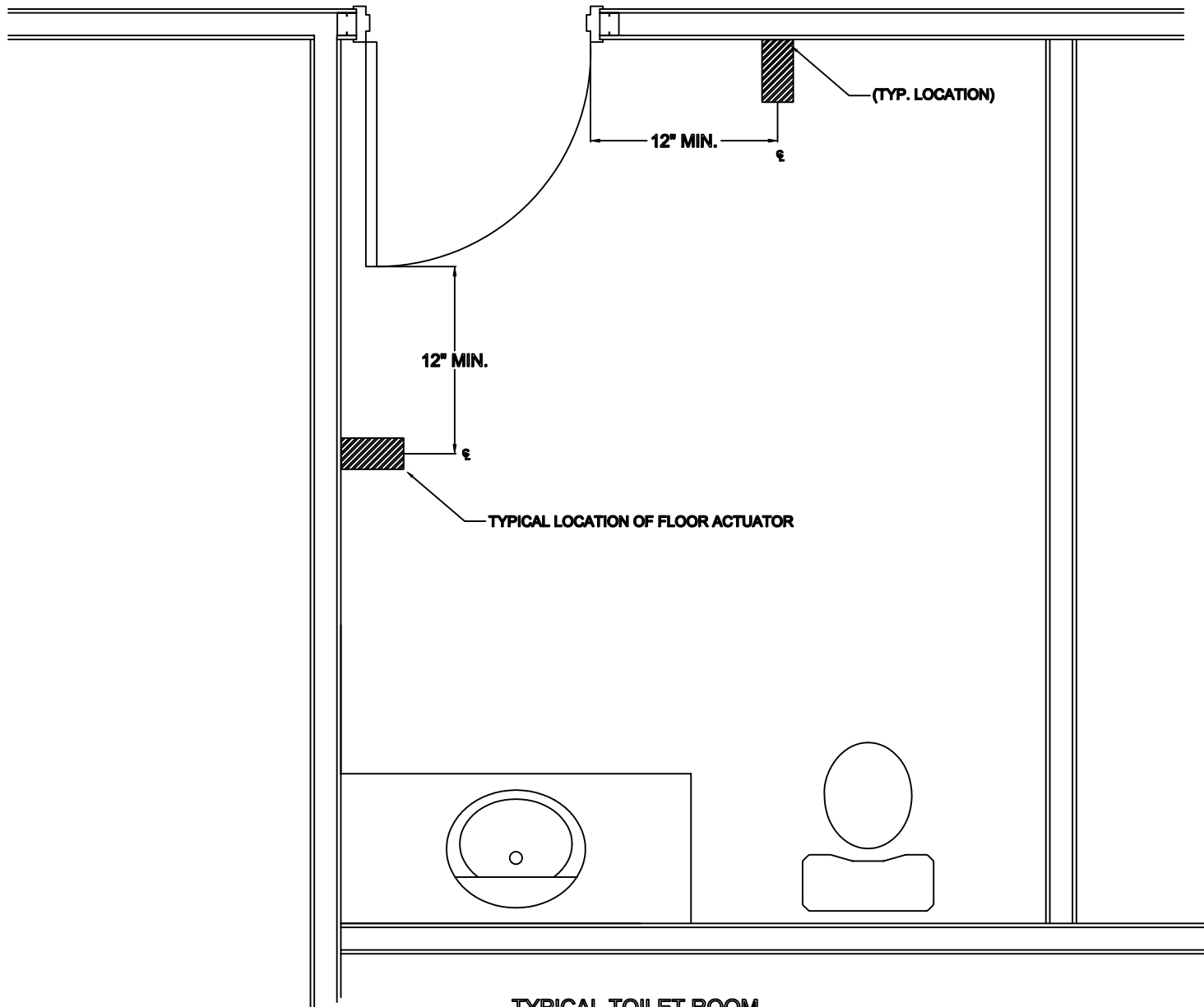
TYPICAL TOILET ROOM
